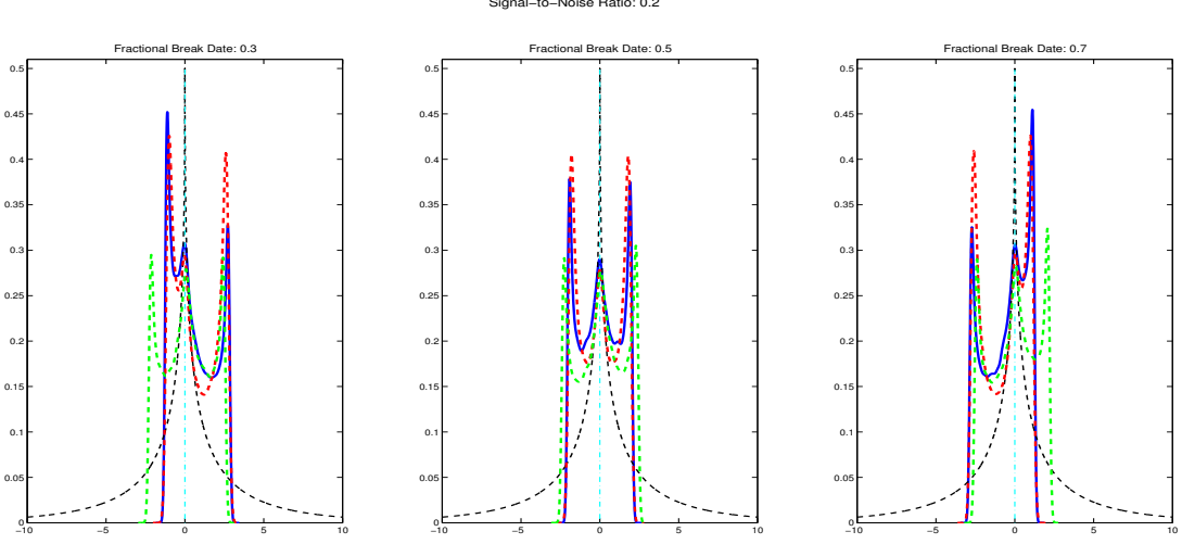
Figure 1: The probability density of \rho(\widehat{T}_{b,\pi} - T_b^0) for model (5.1) with break magnitude \delta_Z^0 = 0.2 and true break fraction \lambda_0 = 0.3, 0.5 and 0.7 (the left, middle and right panel, respectively). The signal-to-noise ratio is \delta_Z^0/\sigma_e = \delta_Z^0 since \sigma_e^2 = 1 . The blue solid (green broken) line is the density of the infeasible (reps. feasible) asymptotic distribution derived under a continuous record, the black broken line is the density of the asymptotic distribution from Bai (1997) and the red broken line is the density of the finite-sample distribution.
