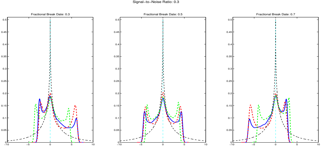
Figure 2: The probability density of \rho(\widehat{T}_{b,\pi} - T_b^0) for model (5.1) with break magnitude \delta_Z^0 = 0.3 and true break fraction \lambda_0 = 0.3, 0.5 and 0.7 (the left, middle and right panel, respectively). The signal-to-noise ratio is \delta_Z^0/\sigma_e = \delta_Z^0 since \sigma_e^2 = 1 . The blue solid (green broken) line is the density of the infeasible (reps. feasible) asymptotic distribution derived under a continuous record, the black broken line is the density of the asymptotic distribution from Bai (1997) and the red broken line is the density of the finite-sample distribution.
